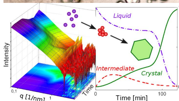
Non-classical nucleation and crystal growth in protein crystallization followed by real-time optical microscopy and SAXS. The sample was beta-lactoglobulin with \text{CdCl}_2 .
